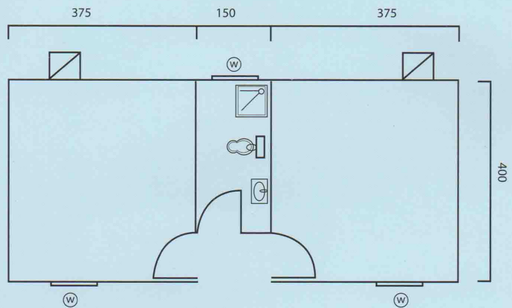
2 ROOMS WITH ONE BATHROOM
