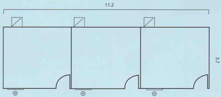
CARAVAN WITH THREE ROOMS
